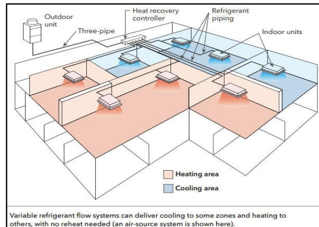
Figure 10: Typical VRF Schematic Diagram
