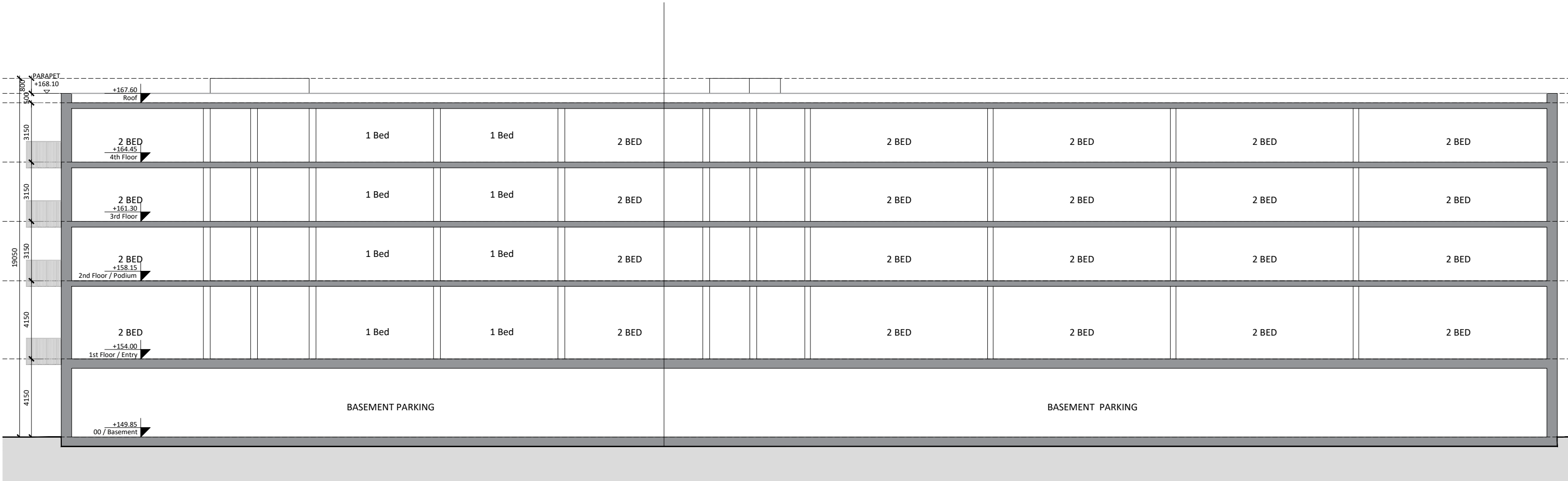
01 — Block C3 - Section BB Scale 1:200
