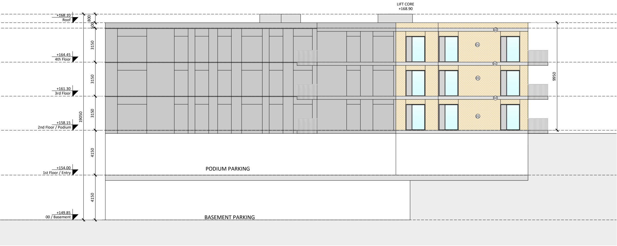
01 — Block C3 - Elevation 04 Scale 1:200
