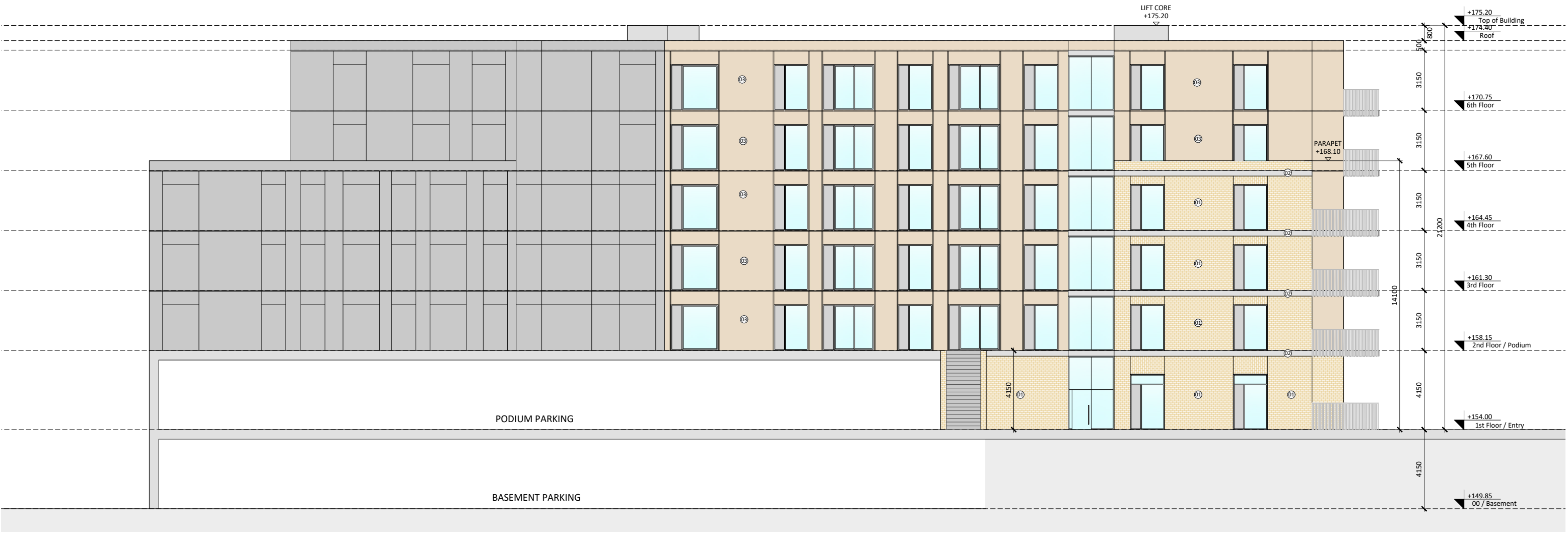
01 — Block C2 - Elevation 06 Scale 1:200
