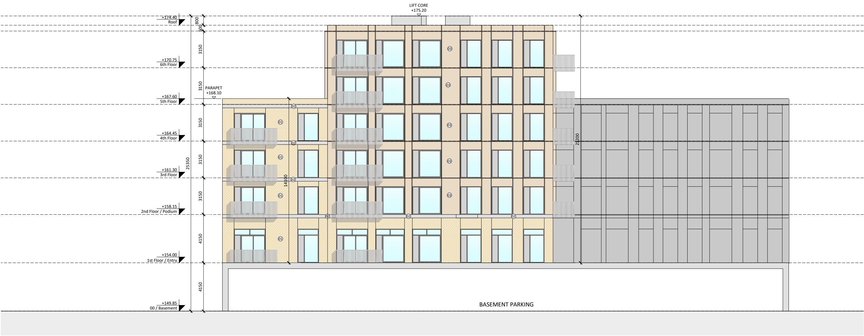
01 — Block C2 - Elevation 01 Scale 1:200
