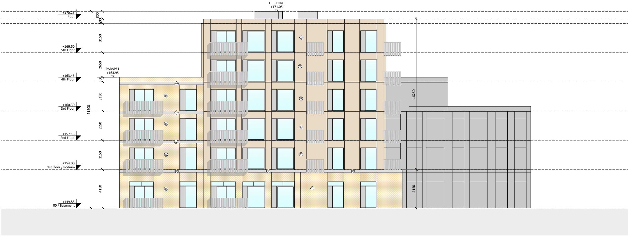
01 — Block C1 - Elevation 01 Scale 1:200
