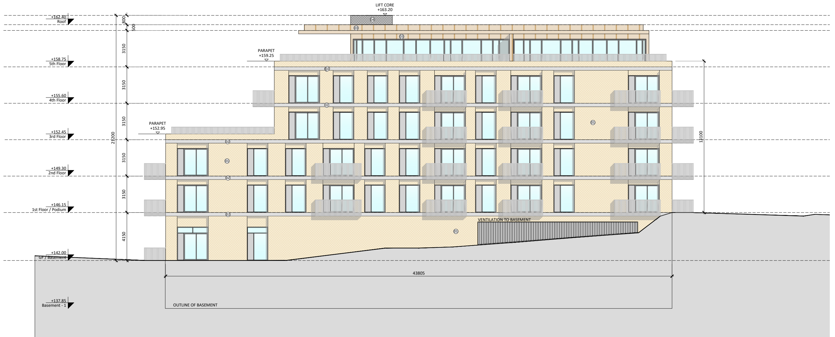
01 — Block B3 - Elevation 03 Scale 1:200
