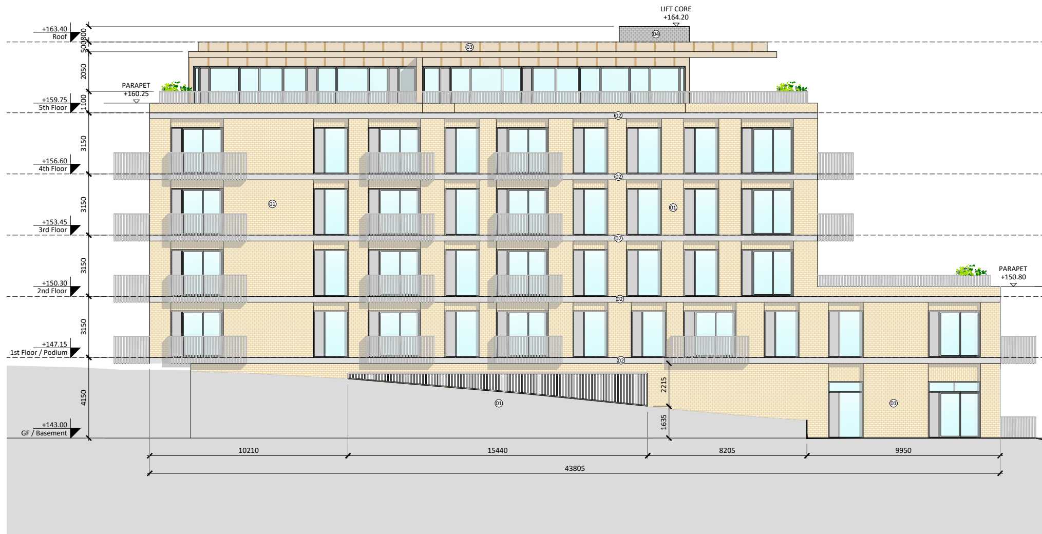
01 — Block B2 - Elevation 01 Scale 1:200
