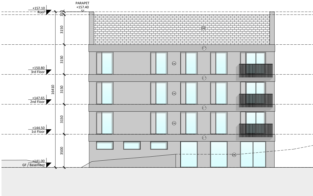
02 Block A1 - Elevation 04 Scale - 1:200
